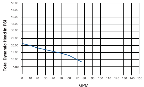
Performance Curve Marathon Motor 7.5 Amp PSI/GPM
