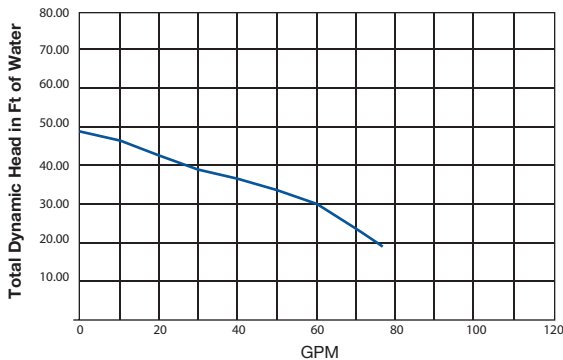
Performance Curve Marathon Motor 7.5 Amp Feet of Water/GPM
